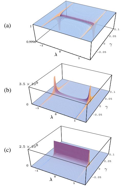
FIG. 2: (color online) (a) The overlap function \langle g(q) | g(\tilde{q}) \rangle , as a function of \lambda and \gamma , for N = 10^6 and \delta\lambda = \delta\gamma = 10^{-6} . Note the clear dips of the plot in the regions of criticality. (b) S_N^\lambda(\lambda, \gamma) . (c) S_N^\gamma(\lambda, \gamma) .
