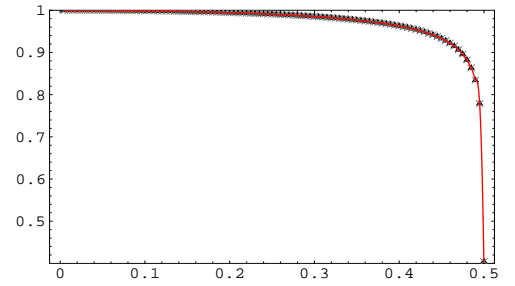
FIG. 1: (color online) The overlap function \langle g | \tilde{g} \rangle , equation (3), as a function of \lambda < \lambda_c , taken for the resonant case \omega_0 = \omega = 1 and \delta\lambda = 10^{-6} . Note the dramatic decreasing of the function as we approach the point of criticality.
