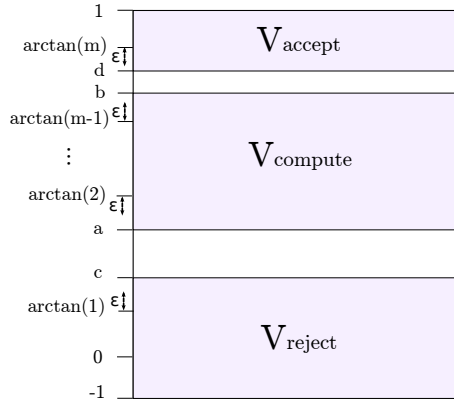
Figure 2: Computing regions for the proof of Theorem 22.
